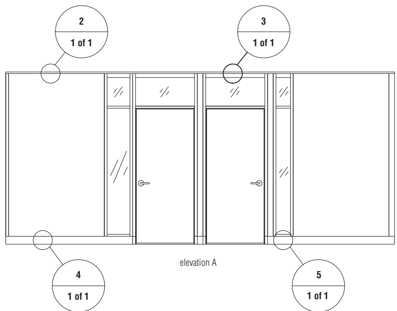
Elevation 1/4" = 1'-0"
