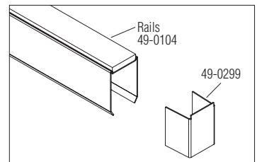
Figure 7 - Recessed End Cap
