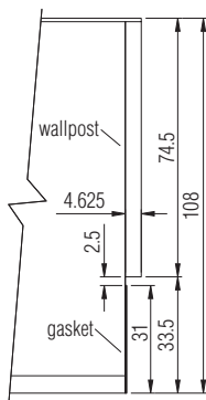
Detail AA
