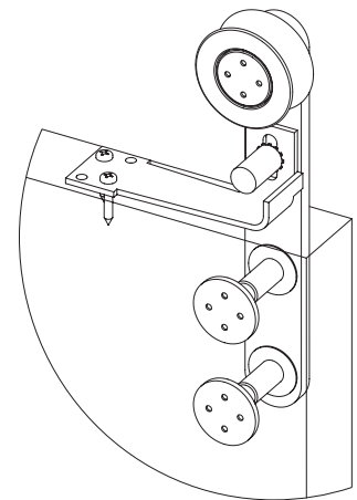
Final Assembly of Wood Door
