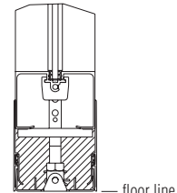
5 glass panel at floor
