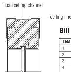
7 glass panel at ceiling
