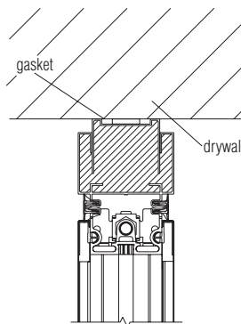
1 solid panel/wallpost at drywall
