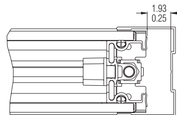
Figure 6 U-Channel
