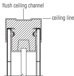
6 solid panel at ceiling
