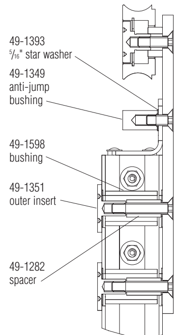
Cross Section of the Final Assembly of Aluminum 3 1/2" Door
