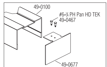
Figure 8 - Flush End Cap
