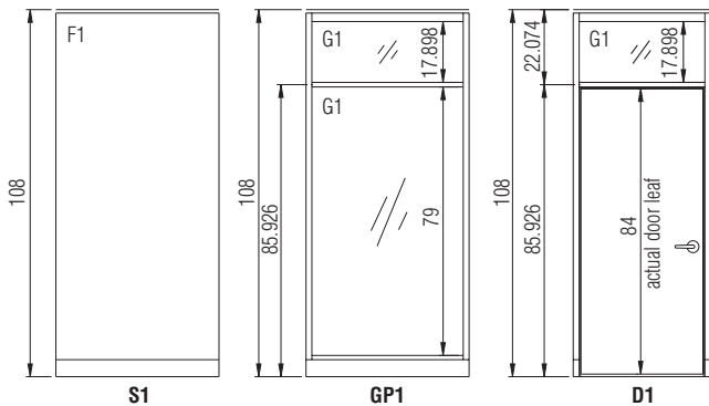
Panel Key 1/4" = 1'-0"
