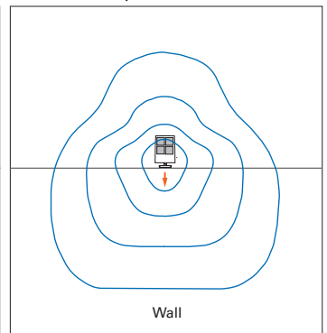
180 - Optics Rotated 180°
