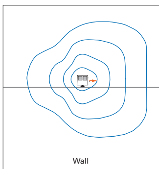
L90 or R90 - Optical orientation for dual pendant
