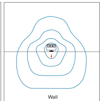
180 - Optics Rotated 180°
