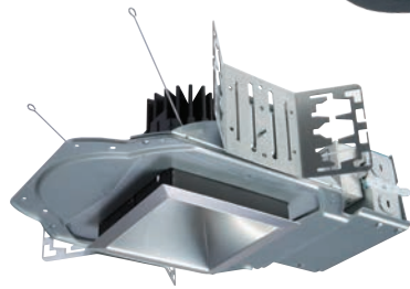
Portfolio LDSQ4B / LDSQ6B 4" and 6" LED downlight
