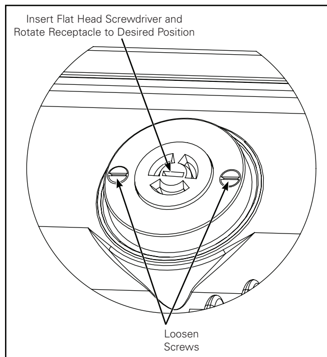
Figure 3. (3-PIN)
