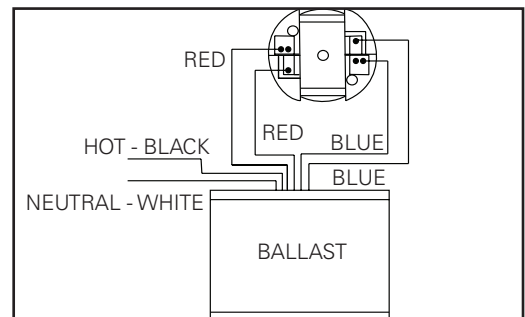
Figure 2. Wiring Diagram
