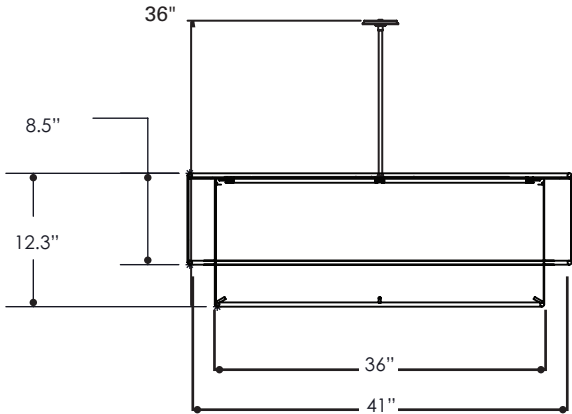
143-36-P1S (SINGLE STEM)
