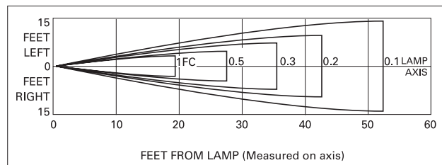
Lamp No. 29-88 Initial Lumens – 29-88 @ 101 Z-4 @ 48
