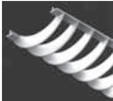
S14 Round Baffle Lateral baffle, 1 1/2" spacing, 35° cutoff, baked white finish.
