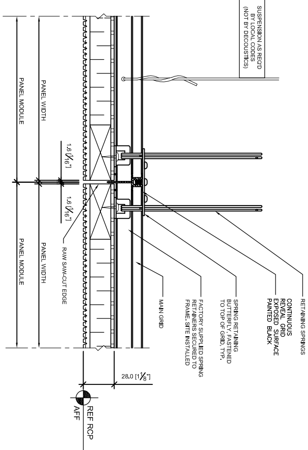
DETAIL @ DEFINED JOINT SCALE 1/2
