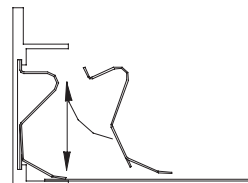
Effects Hold-Down Clip (Item FXSPHDC) for use with cut MetalWorks™ Tegular and Vector® Panels
