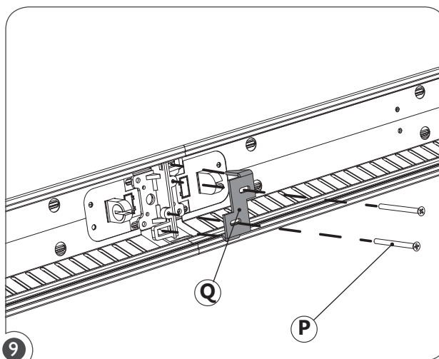
9 Secure the fixtures together using the joining clip (Q) with the supplied screws (P).
