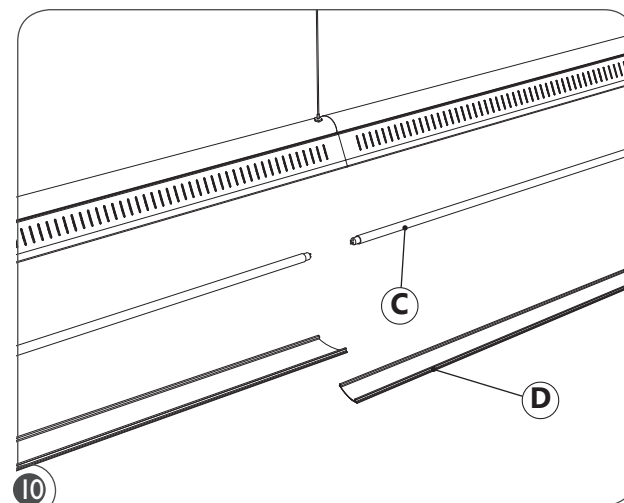
10 Install the lamps (C) and optics (D) in the fixtures.
