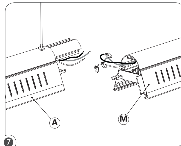
7 CONTINUOUS ROW: If row installation is required, remove lens and lamp if installed in all fixtures. With first fixture (A) in place, repeat steps 3 to 5 with the second fixture (M).
