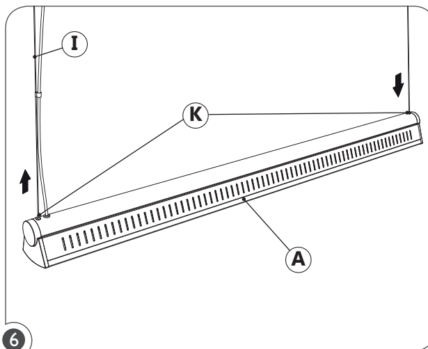
6 To level the fixture, adjust the length of the aircraft cables (I) by pressing down on the cable grip feeder tubes (K). With a level, adjust the fixture (A) so it is straight. BE CAREFUL TO HOLD THE FIXTURE WHILE LEVELING.
