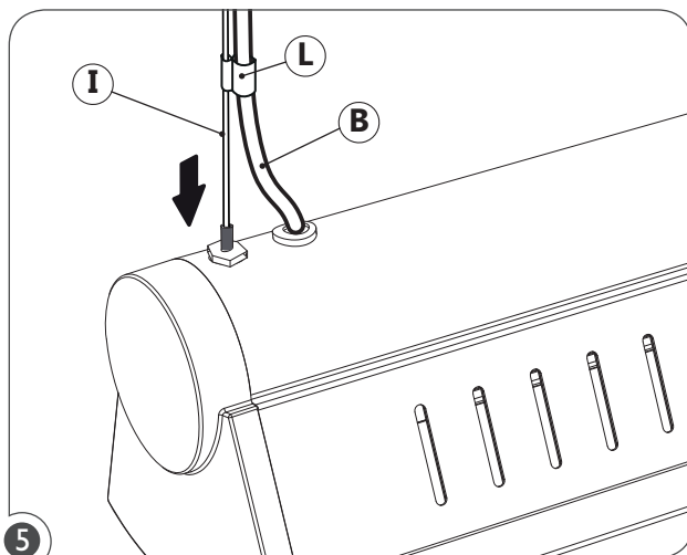
5 Secure power cord (B) to aircraft cable (I) using plastic clips (L).
