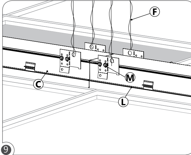
9 Secure the two fixtures using screws (M). Secure support wires (F) to the fixture (L).
