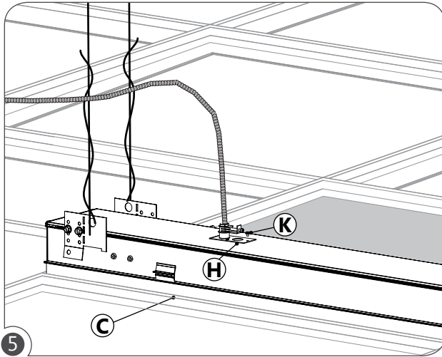
5 Secure knockout plate (H) to fixture (C) by fastening screws (K).
