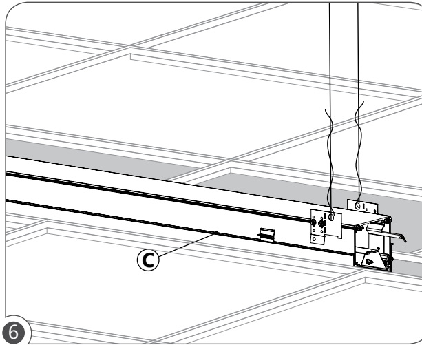
6 CONTINUOUS ROW: Follow steps 1 to 6 for the first fixture (C) in the row.
