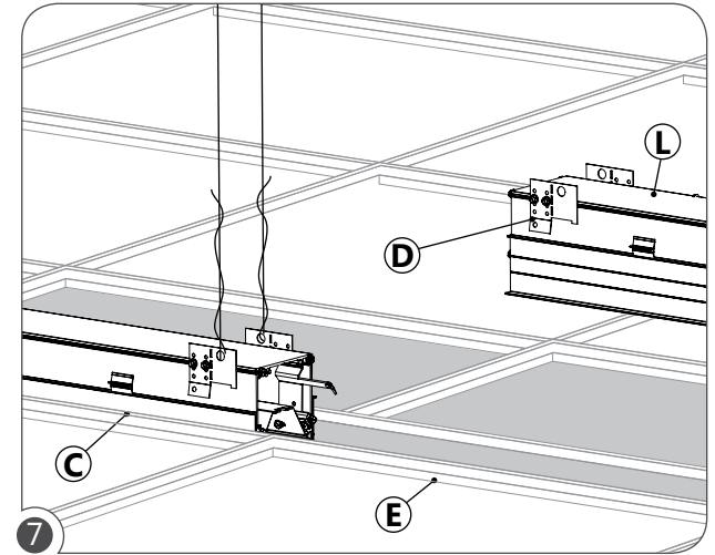
7 Repeat steps 1 and 2 for the second fixture (L). Raise fixture (L) above ceiling, lower fixture onto flanges of T-bars runners (E) from the top. Ensure that safety brackets (D) sit above the T-bars (E).
