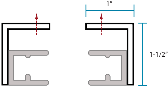
"L" Mullion Leg In
