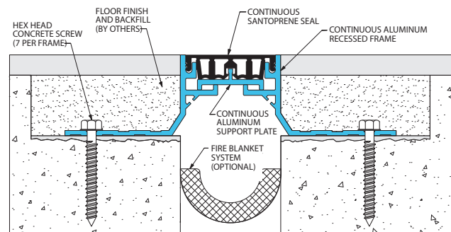
Fire Blanket System (101-A01-050 system shown)
