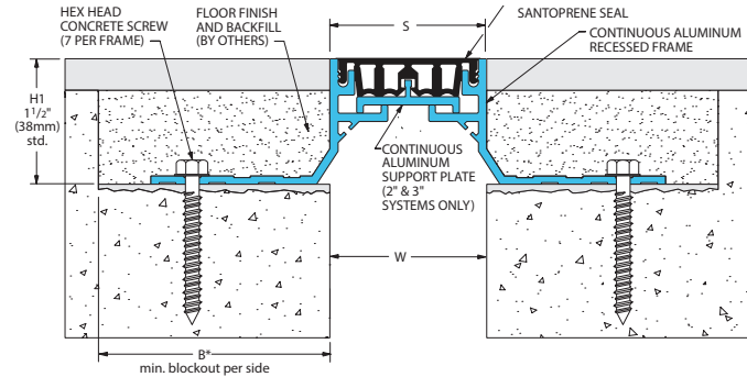
101-A01 Floor/Floor (2" (50mm) system shown)
