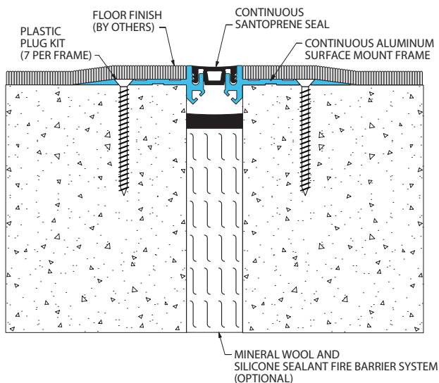
Fire Mineral Wool & Sealant Fire Barrier System (106-A01-025 system shown)
