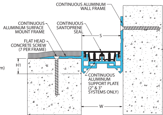
106-A02 Floor/Floor for Carpet (2" (50mm) system shown)
