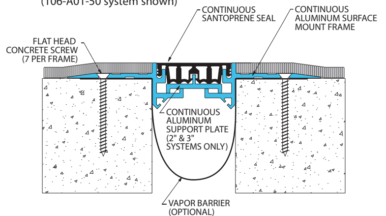
Vapor Barrier System (106-A01-50 system shown)
