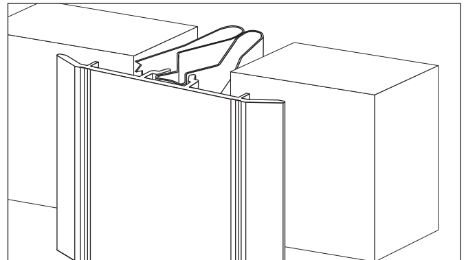
(804-A09 WALL TO CORNER COMPLETED INSTALLATION)
