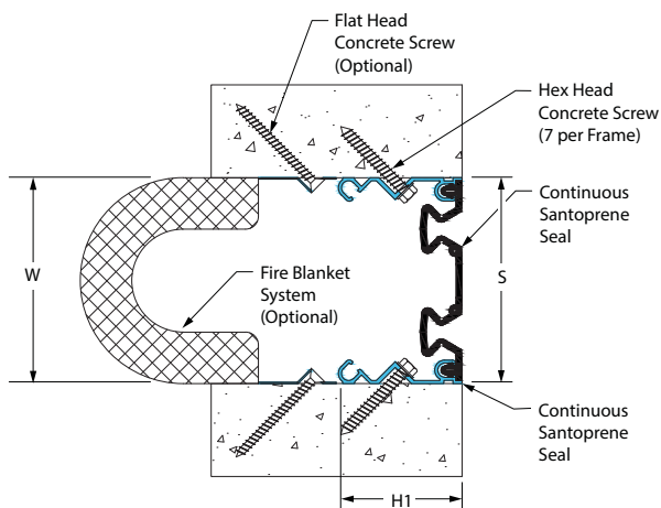
611-A07 Wall/Wall Ceiling/Ceiling (3" (75mm) system shown)
