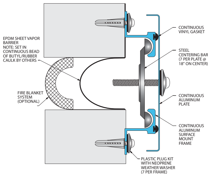
Fire Blanket System (651-A07-050 system shown)
