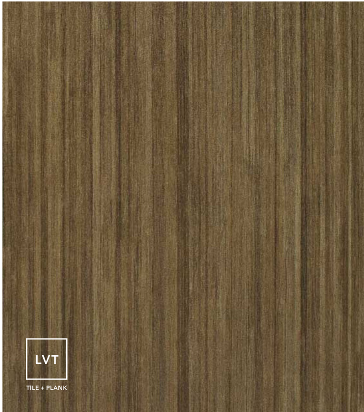
RAYS, ORE
