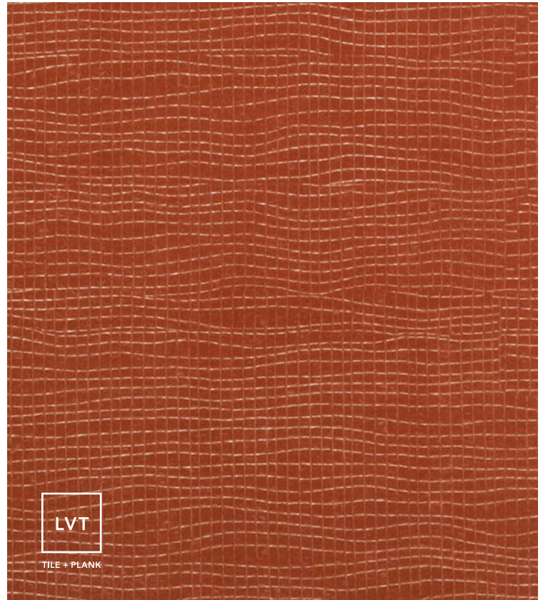
SUBSTRATE, MAGMA
