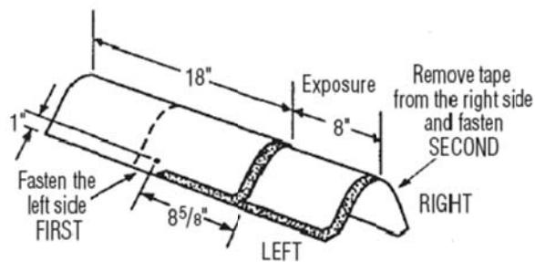
Shangle Ridge – for use with Grand Manor and Carriage House
