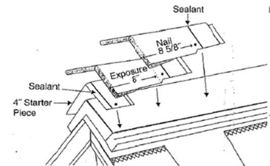
Cedar Crest – for use with Presidential TL, Presidential, Landmark Series incl. TL, Highland Slate and Hatteras
