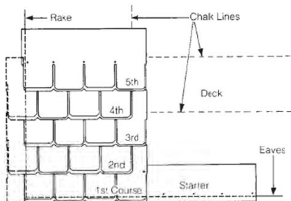
Grand Manor and Carriage House (single column vertical rack method)
