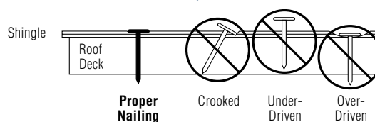
Figure 15-5: Proper and improper nailing.
