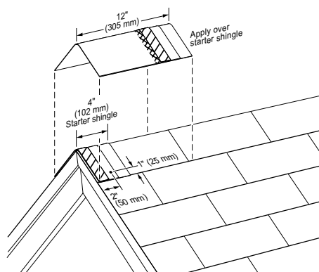
Figure 15-20: Apply a full cap shingle over the starter shingle.
