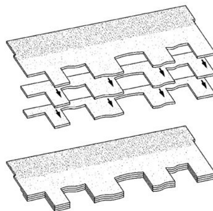
Figure 15-2: Presidential TL Tri-Laminate Construction.
