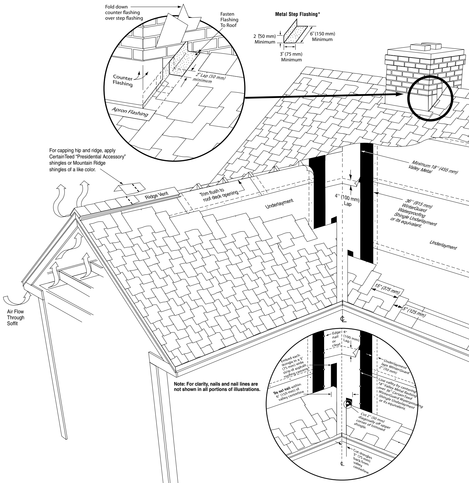
Figure 15-16: Highlight of open valley and chimney flashing details.
