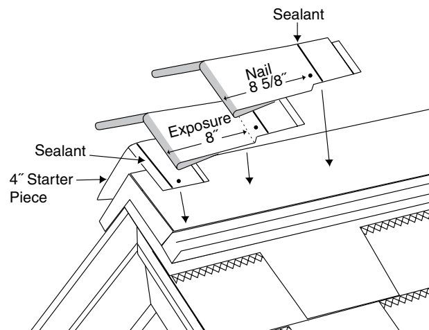
Figure 12-17: Hip and ridge application.
