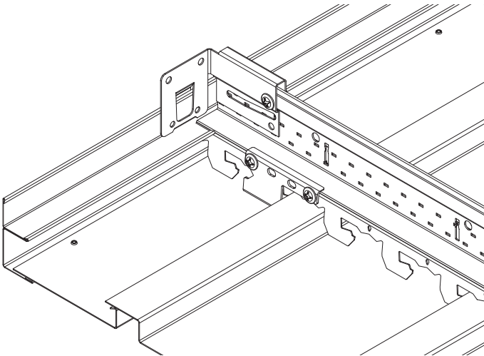
Attached wall, cut plank retaining hook edge
