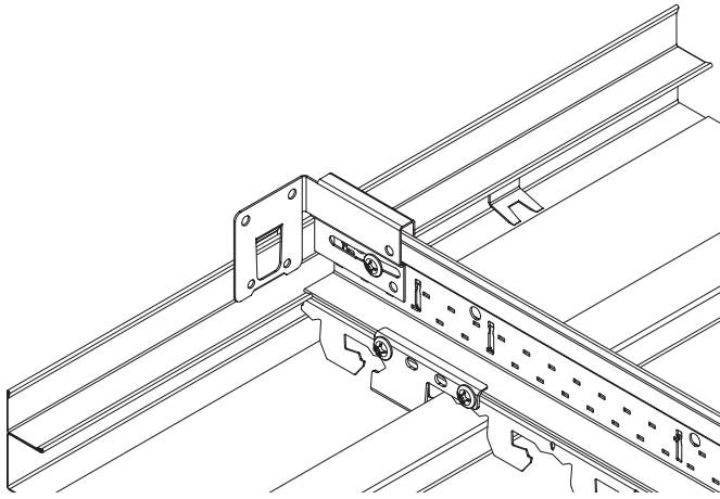
Unattached wall, cut plank retaining flange edge
