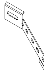
Perimeter Corner Clip (PCC)
