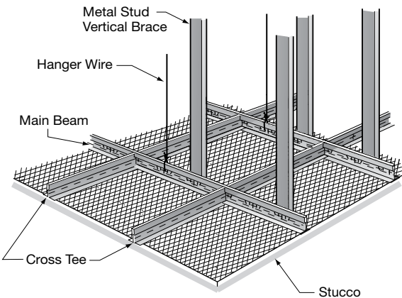
Exterior Wind Loaded Stucco
