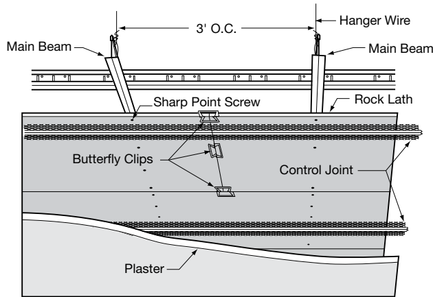
Rock Lath and Plaster
