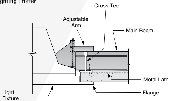
Lighting Troffer
