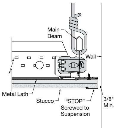
Stucco Perimeter Stop
