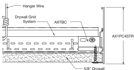
One-Piece Drywall Trim
