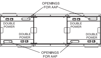
36" DataPath Tech Unit – Front View
