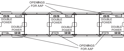
60" DataPath Tech Unit – Front View
