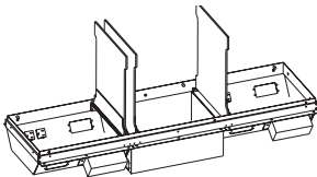
36" DataPath Tech Unit – Open
