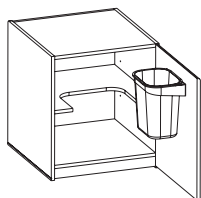
TRS Trash Receptacle with Shelf ($155 upcharge)
