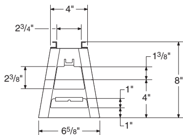
Cable Trough End Dimensions
