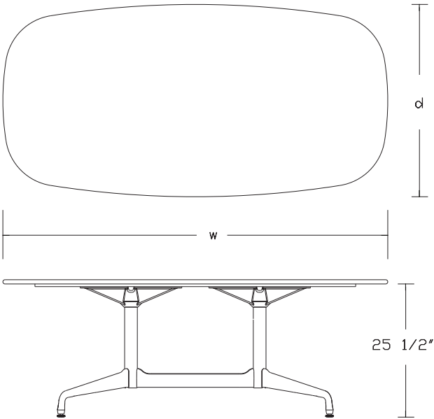
Segmented Base
