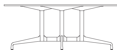
66"-96" Diameter, Segmented Base
