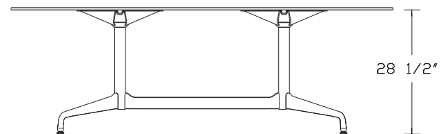
Segmented Base, Width View
