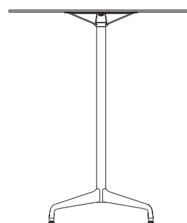
30"-54", Depth View
