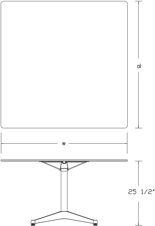
Contract Base
