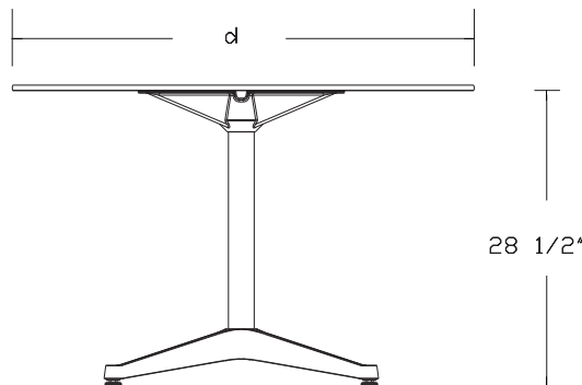
Contract Base
