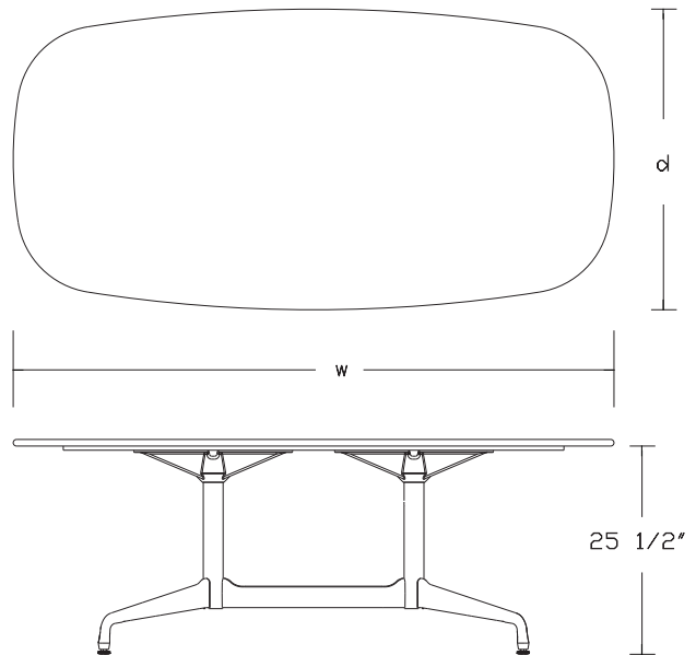
Segmented Base
