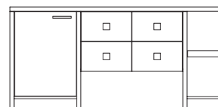
TV CHEST/FRIDGE UNIT LAMINATE TOP ET2376CRM-D-02-L (SHOWN) ET2376CRM-D-02-R (OPPOSITE) D36 W76 H36
