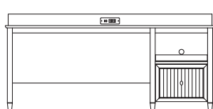
CONSOLE DESK WITH STORAGE CP2373CHD-B-05-L (SHOWN) CP2373CHD-B-05-R (OPPOSITE) D23 W73 H30
