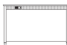
CONSOLE DESK CP1556DKC-B-01-L (SHOWN) CP1556DKC-B-01-R (OPPOSITE) D15 W56 H35
