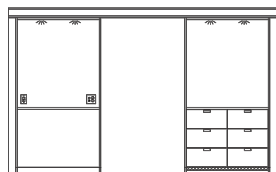
WALL UNIT HUTCH AND DRESSER 12' CT22144WU1 D18 W144 H89.25 14' CT22168WU1 D18 W168 H89.25
