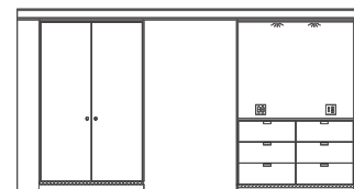
WALL UNIT DRESSER AND WARDROBE 14' CT28168WU3 D24 W168 H89.25
