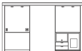
WALL UNIT HUTCH AND MICRO/FRIDGE 12' CT22144WU2 D18 W144 H89.25 14' CT22168WU2 D18 W168 H89.25
