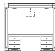
TOWEL SHELF (RECESSED) TD1515TR3 D15 W15 H47.5
