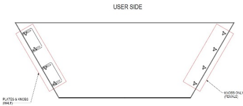
QUICK RELEASE LOCATION "A"
