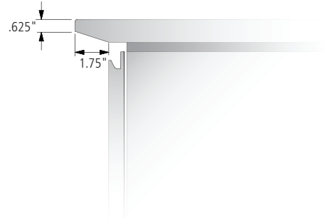
Inset Laminate with Radius Knife (RK) Hardwood Edge
