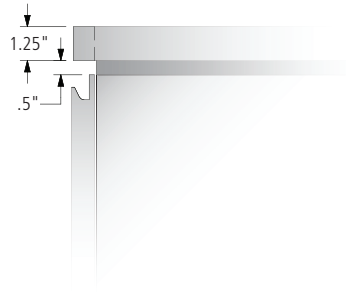
Laminate with Square Hardwood Edge
