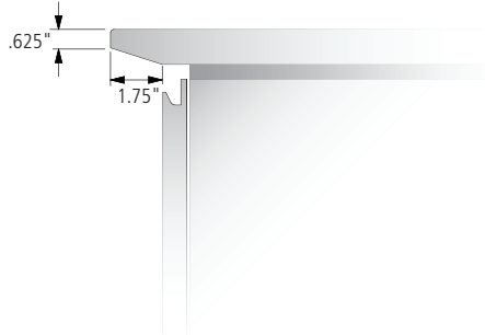
Laminate with Square Hardwood Edge
