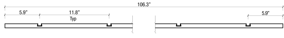
1830-7 US Blade Panel Section View
