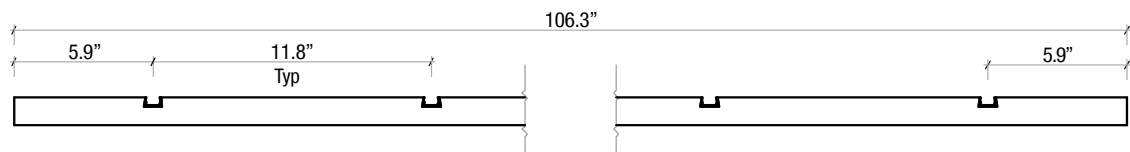
3060-4 US Blade Panel Section View
