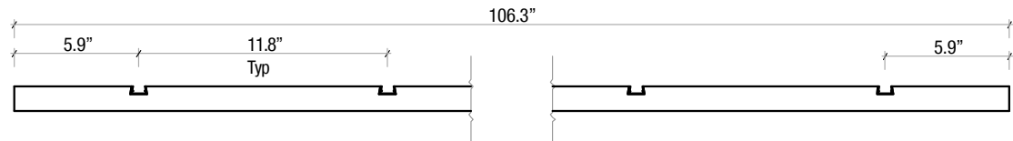
3018-7 US Blade Panel Section View
