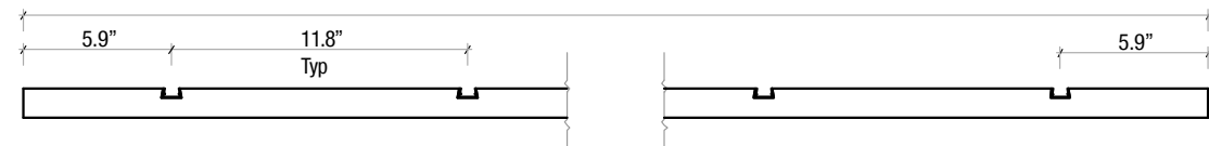
3018-9 US Blade Panel Section View
