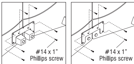
Detail A - Feet
