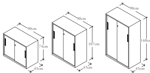
07 sliding door storage cabinet
