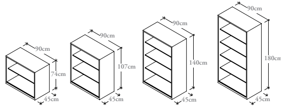
03 swing door storage cabinet
