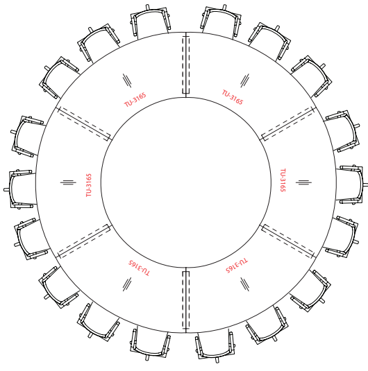
94 1/2 inside dia 165 3/8 outside dia
