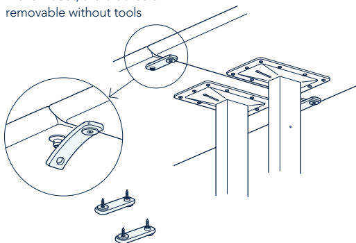
Flexible Ganging Bracket connecting tables that Move About; the bracket is removable without tools
