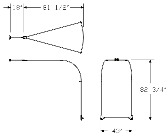
60" Support Arm Length Reference
