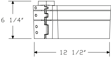
Input Table Leg Attachment
