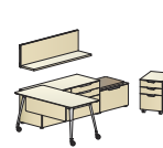
pivoting desk with secondary height credenza and shelf overall dimensions 107.25"W 71.25"D 56"H
