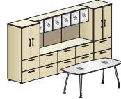
glass desk with primary height workwall and storage units overall dimensions 150"W 109.5"D 69"H
