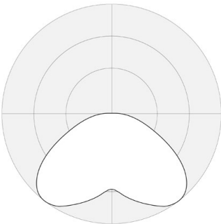
100% Dn Loop Recessed 6" x 1" 4000 K
