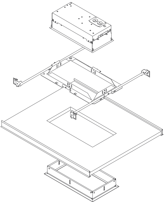
Required Aperture: \frac{6.5" \times 12.5"}{(165 \times 318)}
