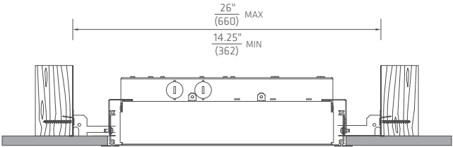
Trim or Trimless (mud-in) Flange Kit
