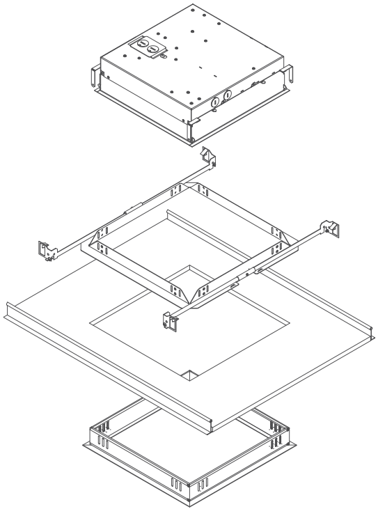
Required Aperture: \frac{12.5" \times 12.5"}{(318 \times 318)}
