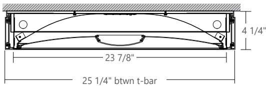
SECTION VIEW
