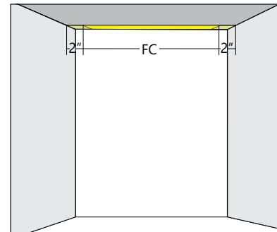
FC: Field cuttable - linear.
