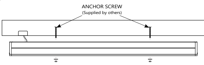
SC SURFACE MOUNT SOLID CEILING
