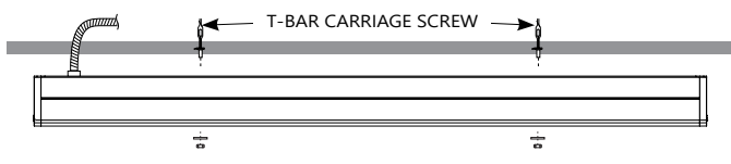
SB9 SB15 SBS SURFACE MOUNT T-BAR CEILING
