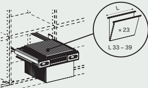
Portacartelle estraibile L 50 /Filling pull-out frames L 50
